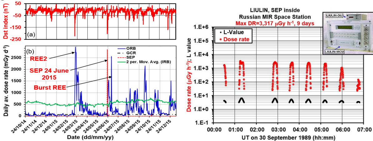
Figure 1a. Daily Dst index variations; Figure 1b. Daily GCR, IRB, ORB and SEP dose rate variations as measured by R3DR2 instrument on Russian segment of ISS. Some of the extreme events studied in the paper are marked. Figure 2. External view of the LIULIN dosimeter radiometer and dose rate data dynamics during the SEP on 30 September 1989.
