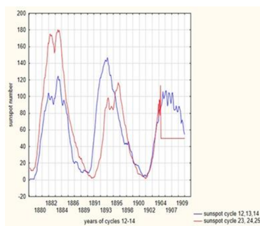
Figure 3. Evolution of cycles 23, 24 and the beginning of 25.
