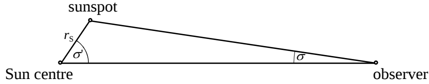
Fig. 2: with known distance between observer and the Sun ( d_{\text{observer-S}} ), apparent angular distance between centre of the Sun and sunspot ( \sigma ) and Solar radius ( r_s ), angle ( \sigma' ) can be determined, as well as heliocentric coordinates of sunspot.
