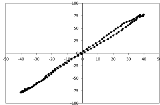
Fig.4. Y_1 vs. Y_2 (12-month running means) along an 11-year cycle.
