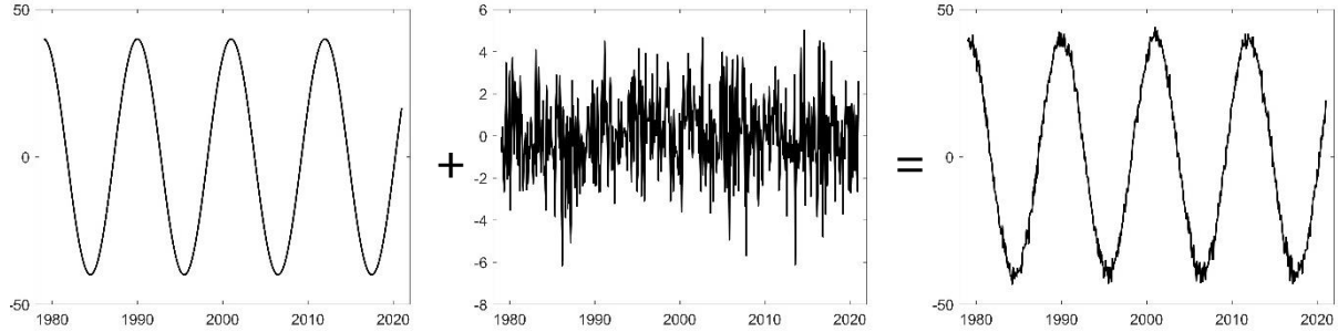
Fig.2. Schematic representation of an artificial series generated to simulate an EUV proxy (right panel), that results from the sum of \cos(2\pi t/11) (left panel) (with 40 units amplitude) and a random noise (middle panel).
