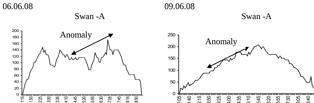
Fig.3. The time – series of the ionosphere field (Shooshi station) obtained by Radio astronomical method for BORISAKHO (Georgia, 09.06.08, M=4.1 ) the earthquake.
