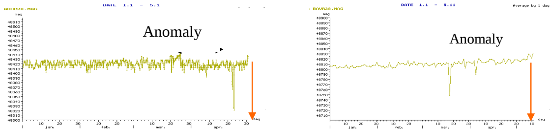
Fig.2. The time – series of the geomagnetic field (Aruch, Bavra stations) for the VARDENIS (Armenia, 29.04.2008, M=3.7 ) earthquake.
