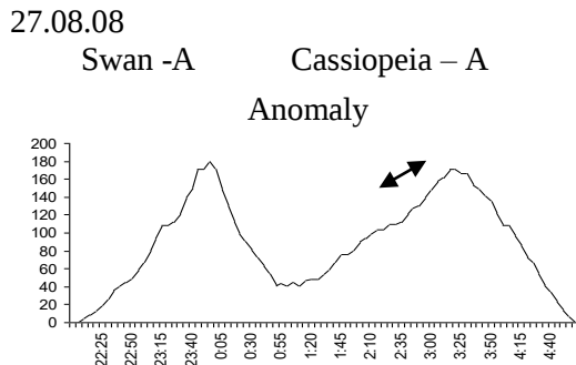
Fig.4. The time – series of the ionosphere field (Saravand station) obtained by Radio astronomic method for the NAKHITCEVAN (Azerbaijan, 02.09.2008, M=5.1 ) earthquake.
